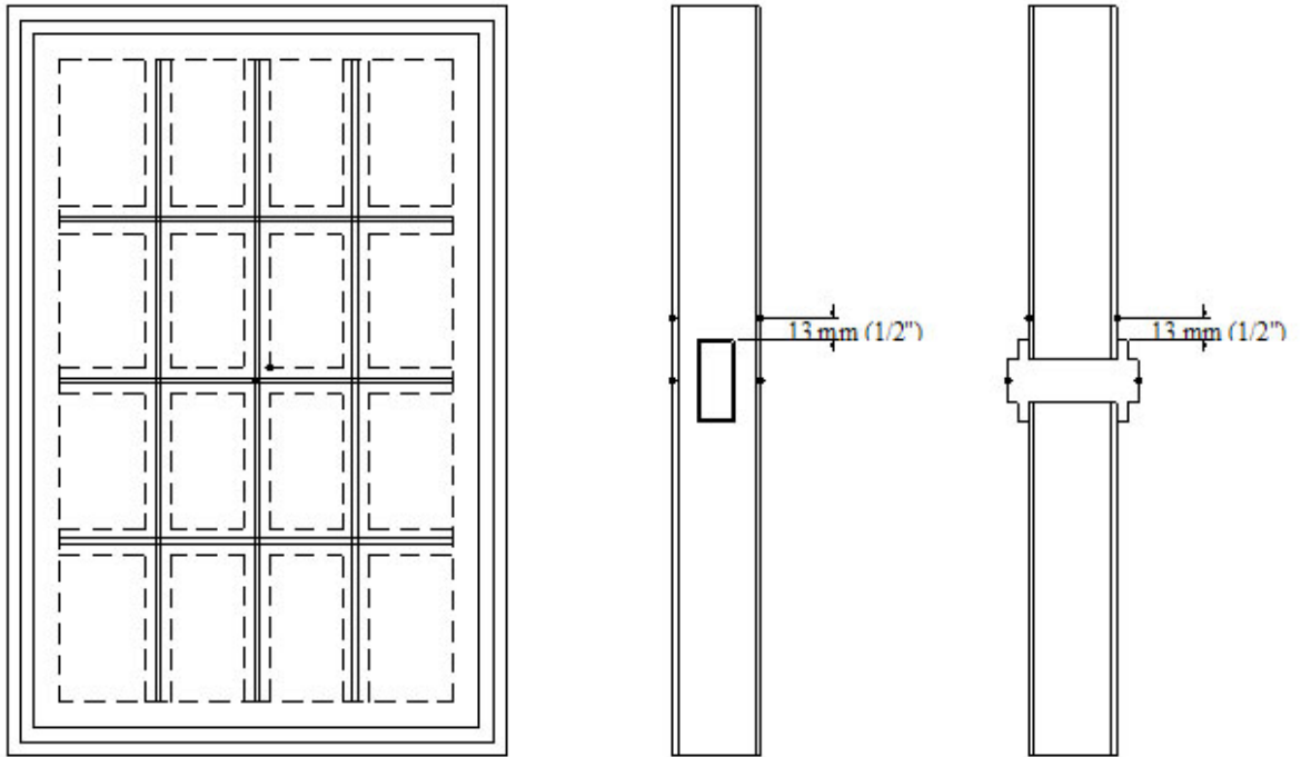
Figure 6-6 Divider Thermocouple Placement
