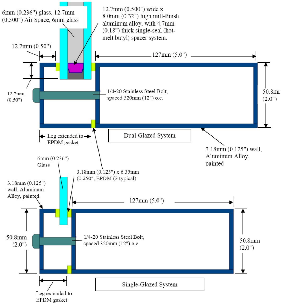
Figure 5-4 Cross Section B
