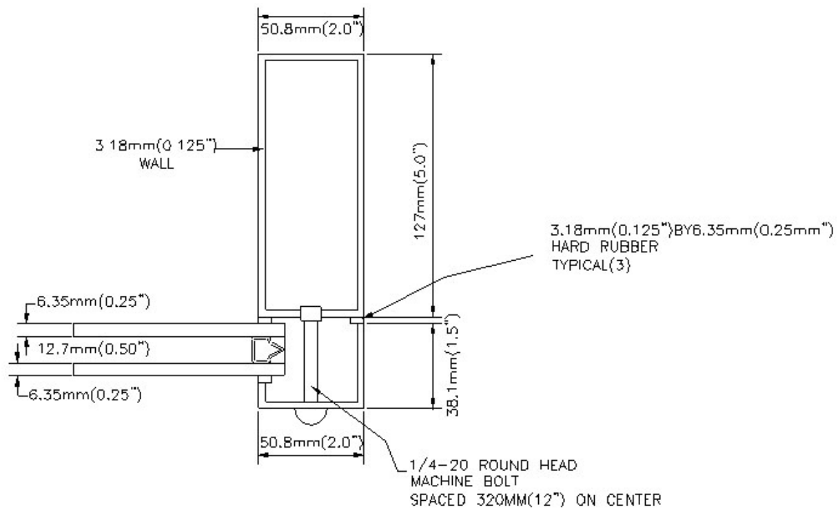
Figure 5-5 Cross Section B
